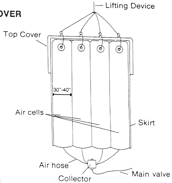
X-Sectional View
